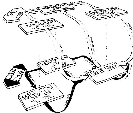
Figure 2.4 The four cornerstone equations for the two-fluid model with equal pressure of the two phases.
