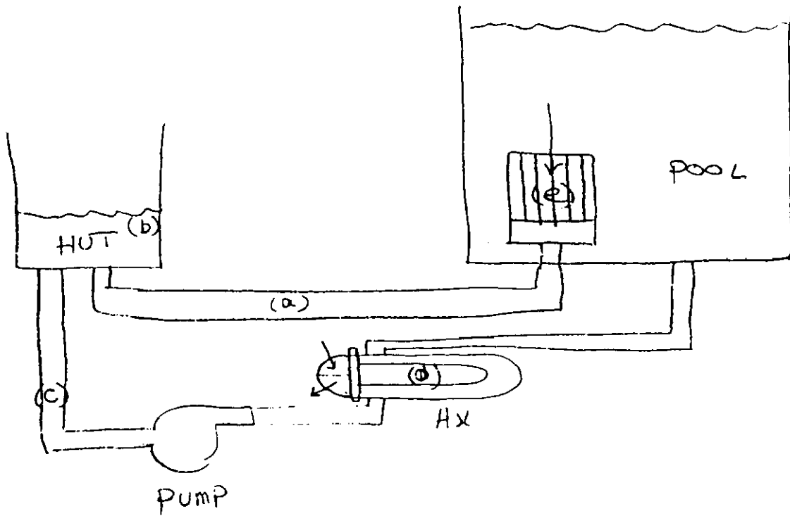
Figure 2.5 Simple pool-type research reactor.
