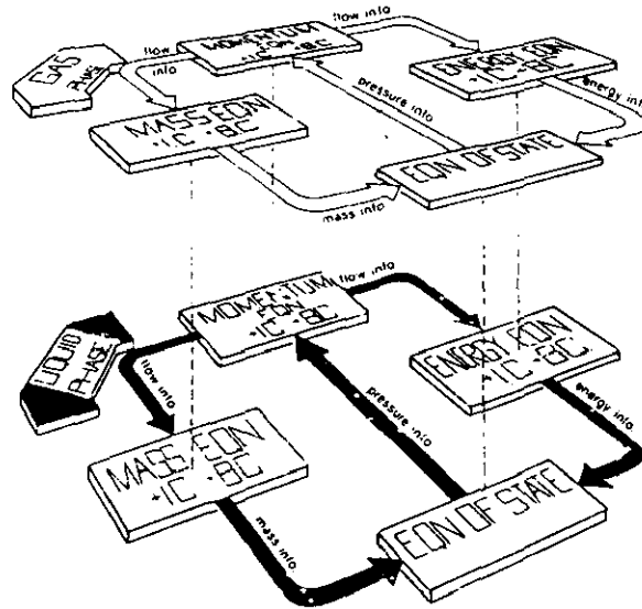
Figure 2.3 The four cornerstone equations for the full two-fluid model.
